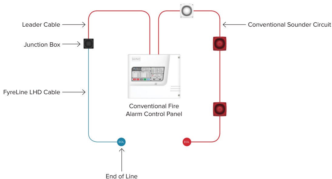
Figure 2: Typical Wiring Configuration Conventional System
