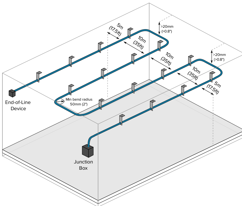
Figure 10: Protecting large areas with LHD cable
